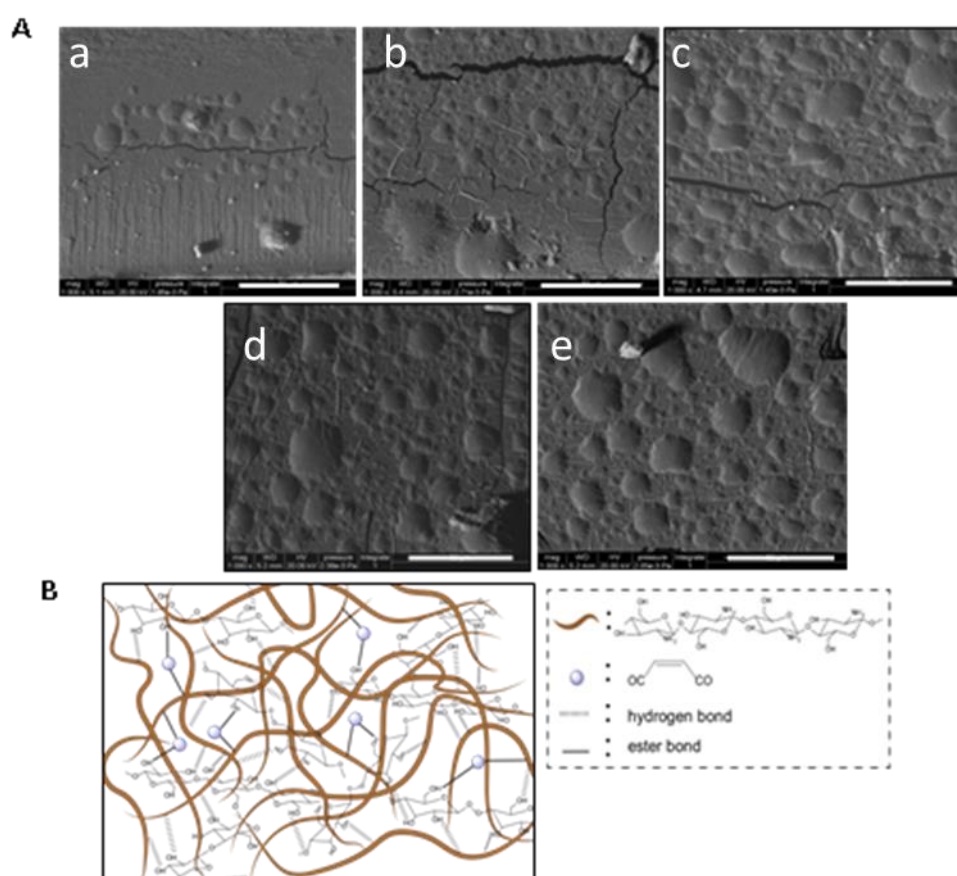
Figure 3. A. SEM photographs (1000× amplification) of starch film (a), S/CH 3% film (b), S/CH 7% film (c), S/MA-CH 3% film (d), S/MA-CH 7% film (e); B. illustrative scheme of S/MA-CH films. Scale bars indicate 50 \mu\text{m} .
